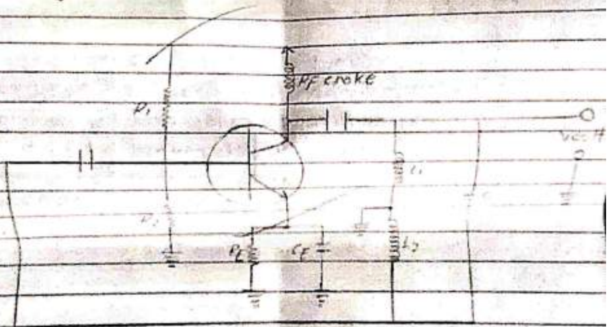
Fig.1 Hartley oscillator.
