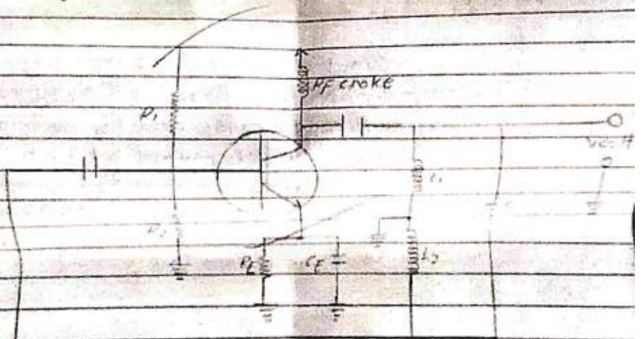
Fig. 1 Hartley oscillator.
